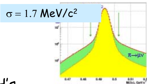
(\pi^{\pm} \pi^{\pm} \pi^{-}) mass GeV/c^2
