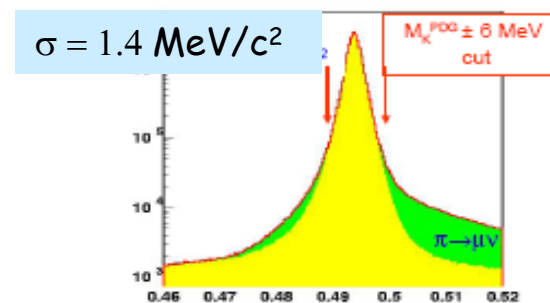
(\pi^{\pm} \pi^0 \pi^0) mass GeV/c^2
