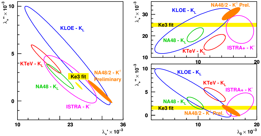
Abbildung 2: Quadratic fit results for K_{\mu 3} ( K_L for neutral and K^\pm for charged) decays. The ellipses are the 1 \sigma contour plot. For comparison also the K_{e 3} fit from FlaviaNet WG1 is shown.
