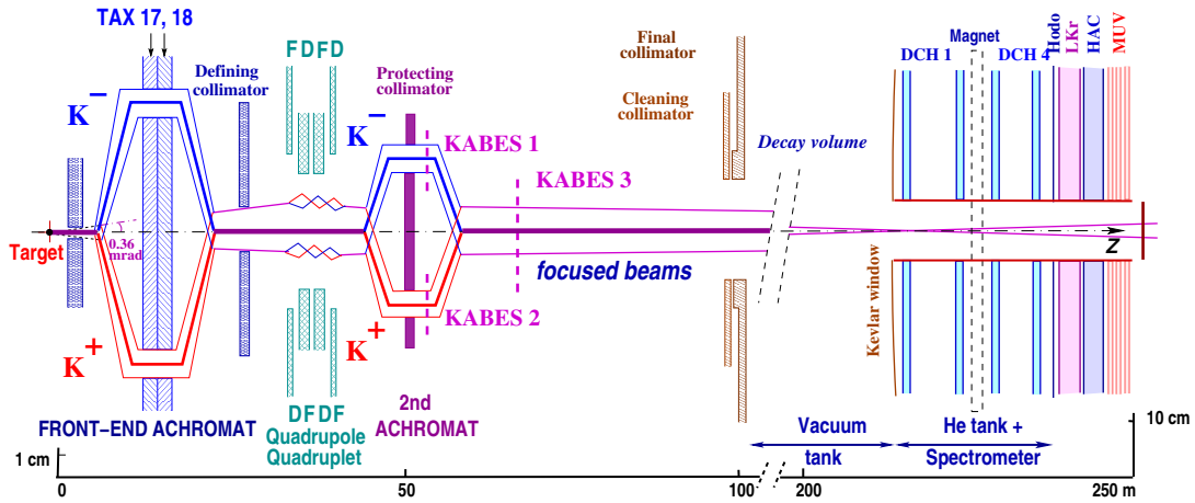
Abbildung 1: Schematic side view of the NA48/2 beam line, decay volume, and detectors.
