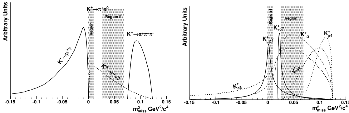
Figure 2: Squared missing mass for Kaon decays. The squared missing mass is defined as the square of the difference between the 4-momentum of the kaon and of the decayed track in the hypothesis that it is a pion.
