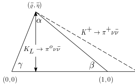
Figure 2: Connection between the branching ratios of K \rightarrow \pi\nu\bar{\nu} decays and the unitarity triangle.
