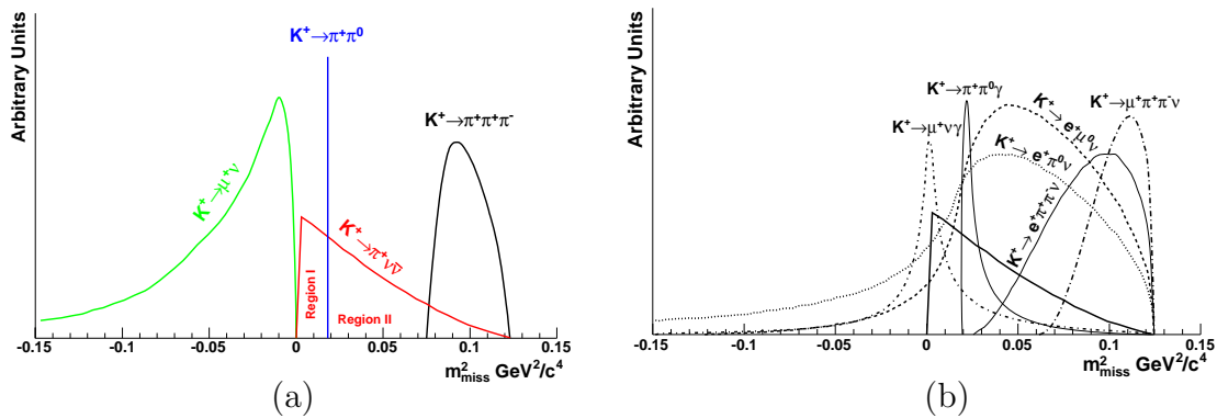
Figure 3: Kinematically constrained (a) and kinematically not constrained (b) backgrounds to K^+ \rightarrow \pi^+ \nu \bar{\nu} decays.
