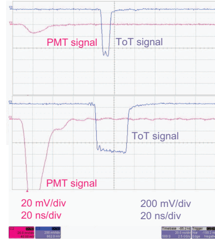
Figure 3: Analog signal from PMT and LVDS signal from time-over-threshold discriminator for two muon signals, ranging from \sim 20 (top) and \sim 600 mV/ \Omega (bottom).
