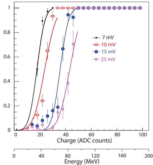
Figure 5: TDC efficiency as a function of signal amplitude (recorded by the charge ADC) for four different values of the threshold of time-over-threshold discriminator. Taking into account the MIP energy deposit ( \sim 80 MeV) and the MIP/ADC calibration factor, the corresponding energy scale has been calculated.
