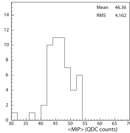
Figure 4: Average values of MIP for all equipped lead-glass crystals for a muon run in NA62 (summer 2009). The HV settings were adjusted on the basis of cosmic-rays data. The mean of 45 ADC counts corresponds to 4 pC, well matching what is expected for a gain of \sim 10^6 , the RMS is at 10% level.
