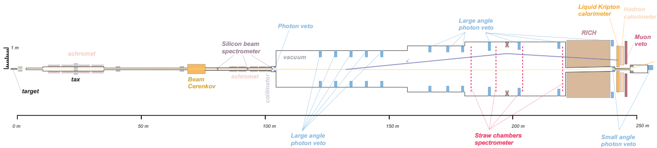
Figure 1: Schematic layout of the NA62 experiment. The 12 LAV stations all along the decay vacuum tube are shown.
