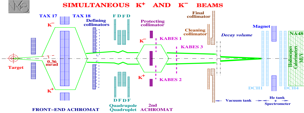
Figure 1. Schematic vertical section of the simultaneous K^+ and K^- beam line (not to scale).
