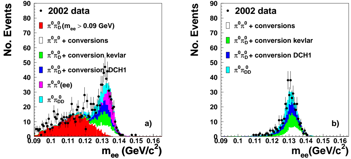
Figure 2: Distributions of m_{ee} after all the cuts have been applied. Superimposed we show the Monte Carlo predictions from all important sources. Figure a) shows the components with opposite-sign tracks; figure b) shows the ones with same-sign tracks.
