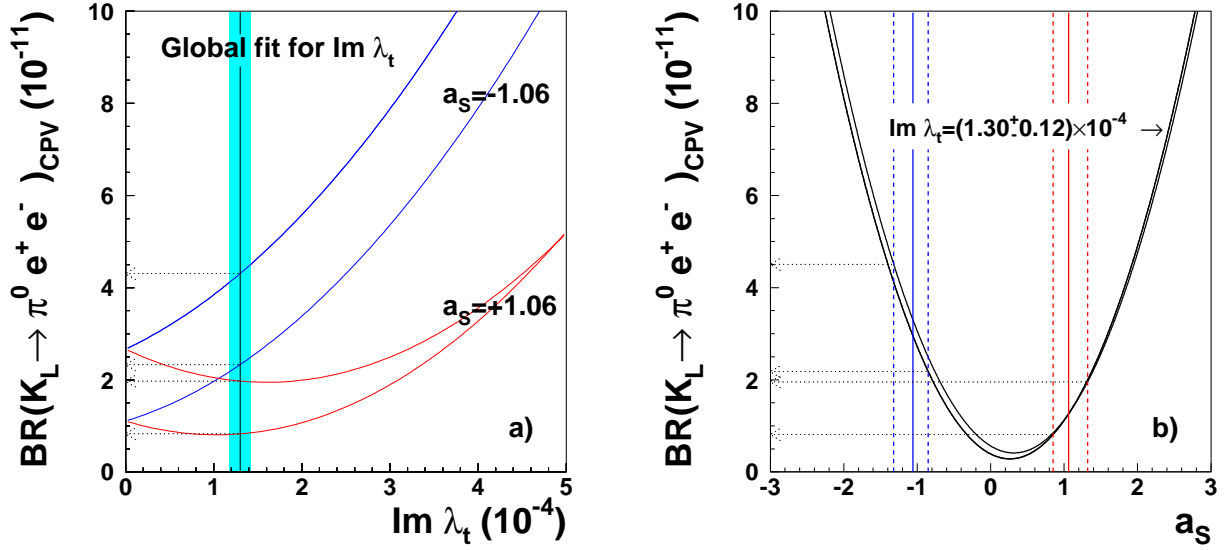
Figure 7: Branching fraction of K_L \rightarrow \pi^0 e^+ e^- as a function of \text{Im}(\lambda_t) (a), and as a function of the parameter a_S (b).
