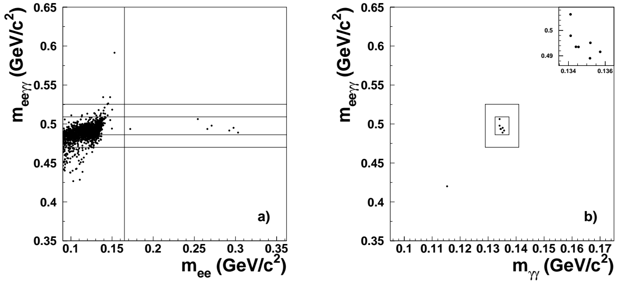
Figure 4: Scatter plot of m_{ee\gamma} versus m_{ee} (a) and m_{ee\gamma} versus m_{\gamma\gamma} (b) for events passing all the cuts described in the text. The regions of 3\sigma and 6\sigma are shown.
