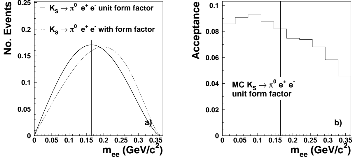
Figure 6: m_{ee} distributions from Monte Carlo, with and without the form factor (a); acceptance as a function of m_{ee} (b).
