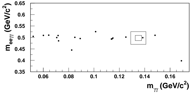
Figure 3: Scatter plot of m_{ee\gamma\gamma} versus m_{\gamma\gamma} for events selected as K_L \rightarrow e^+e^-\gamma\gamma in the 2001 data. The boxes are representing the 3\sigma and 6\sigma regions.
