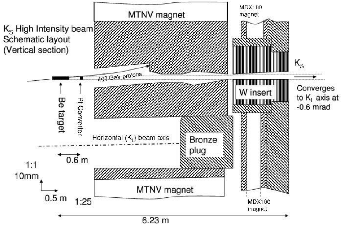
Figure 1: View of the 2002 modifications to the beam line.
