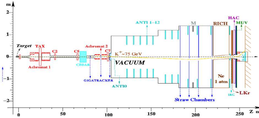
Fig. 2. – The NA62 detector layout.
