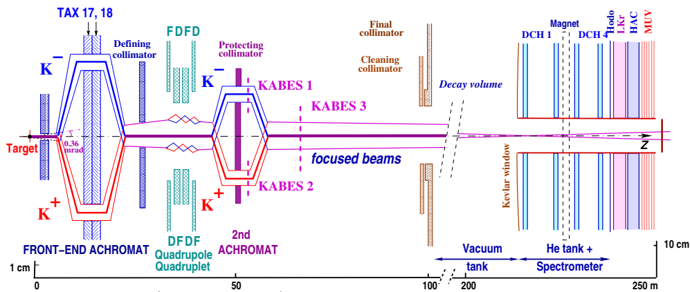
Figure 1: A view of NA48/2 beam line (TAX17,18: motorized beam dump selecting momentum of K^+/K^- beams; DFDF: focusing quadrupoles, KABES1–3: beam spectrometer and detector (DCH1–4: drift chambers, Hodo: hodoscope, LKr: EM calorimeter, HAC: hadron calorimeter, MUV: muon veto). Vertical scale differs in two parts of the figure.
