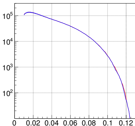
Figure 6: Numbers of observed (red) and expected (blue) DP candidates in the DP signal mass window as for each assumed DP mass hypothesis.
