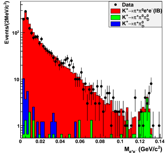
Figure 2: Reconstructed e^+ e^- invariant mass distributions of the data and simulated background samples.
