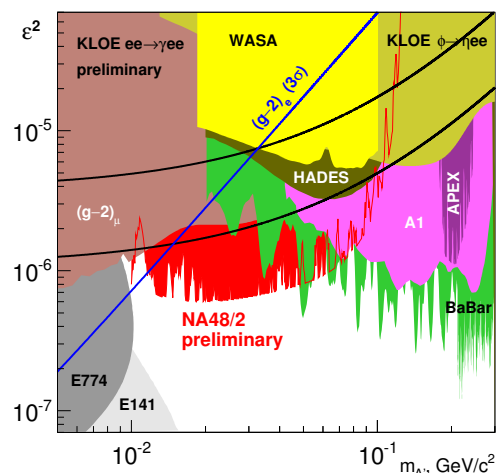
Figure 7: The NA48/2 preliminary upper limits at 90% CL on the mixing parameter \varepsilon^2 versus the DP mass m_{A'} , compared to the other published exclusion limits.
