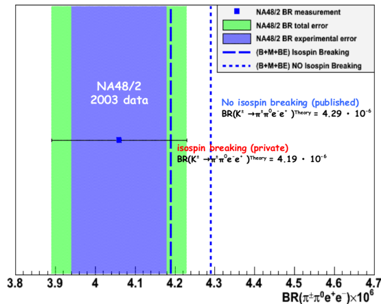
Figure 3: The K^\pm \rightarrow \pi^\pm \pi^0 e^+ e^- preliminary branching ratio is plotted with its experimental error (shaded blue band) and its total error (shaded green band).
