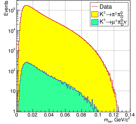
Figure 5: Reconstructed e^+e^- invariant mass distributions of the data and simulated K_{2\pi D} and K_{\mu 3 D} samples.
