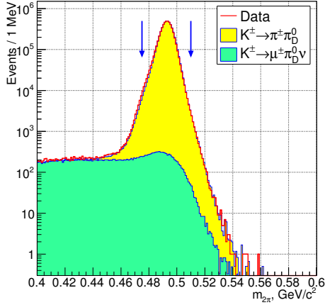
Figure 4: Reconstructed \pi^{\pm}\pi_D^0 invariant mass ( m_{2\pi} ) distributions of the data and simulated background samples. The selection condition is illustrated with arrows.
