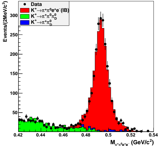
Figure 1: Reconstructed \pi^\pm \pi^0 e^+ e^- invariant mass distributions of the data and simulated background samples.
